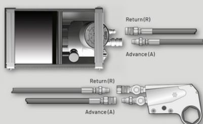
Connection scheme hydraulic hoses
