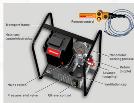
Hydraulic torque wrench alkitronic® H-AT
